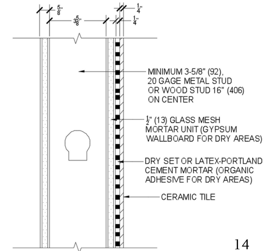
1. THIN-SET CERAMIC TILE 6"=1'-0"
